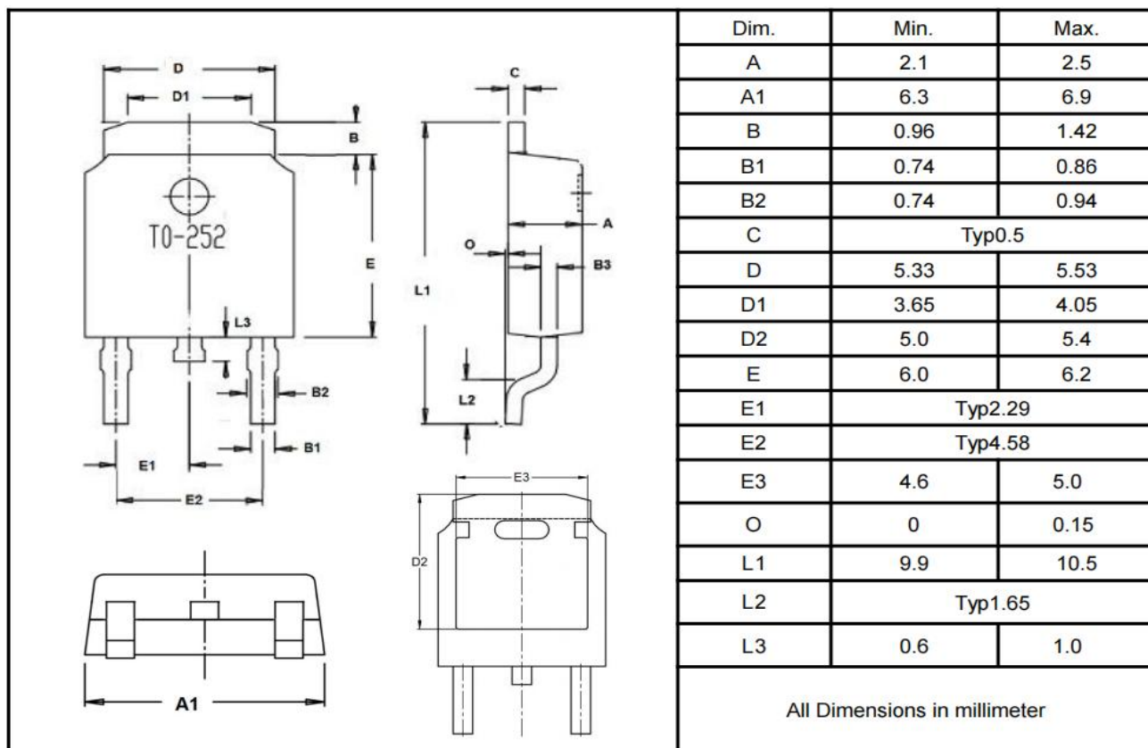
T0-252
