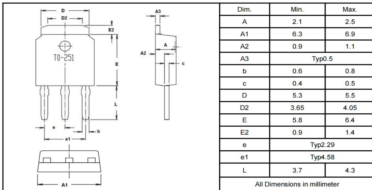
T0-251
