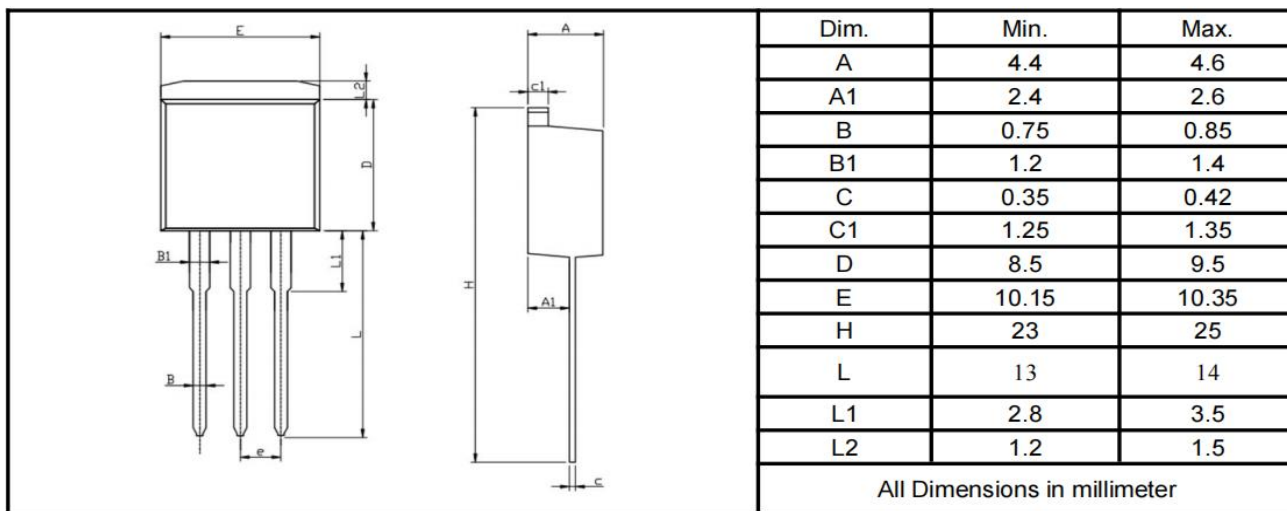
T0-262
